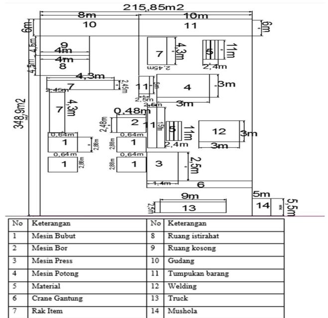
Gambar 1. Layout Pabrik Awal
