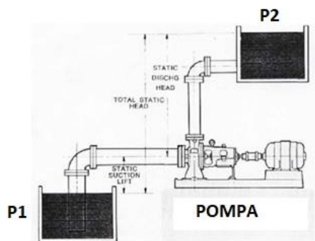
Gambar 6. Head statis total
