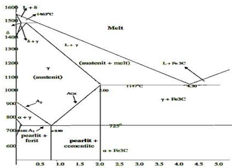
Gambar.3. Diagram Besi Karbon (Fe-C) (sumber: en.wikipedia.org)
