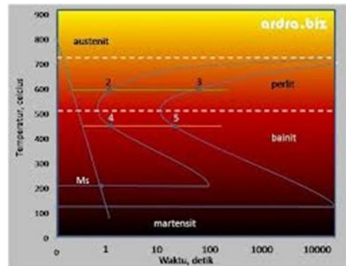
Gambar.11 Diagram TTT
