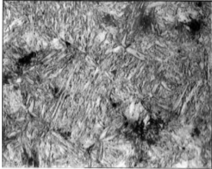
Gambar.8 Martensit (sumber: en.wikipedia.org)
