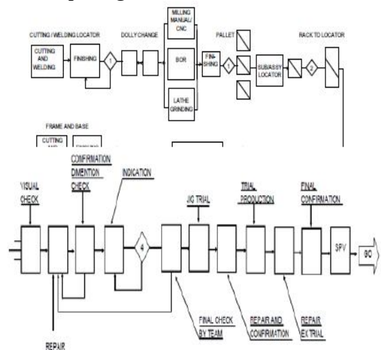
Gambar 3.4. Fabrication Flow Process .
