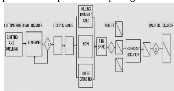
Gambar 3.7. Welding locator fabrication flow process
