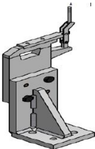
Gambar 3.2 locator Type B
