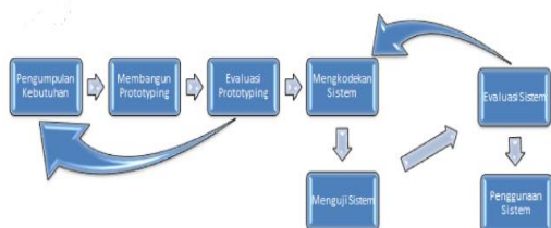
Gambar 2. Metode Prototype
