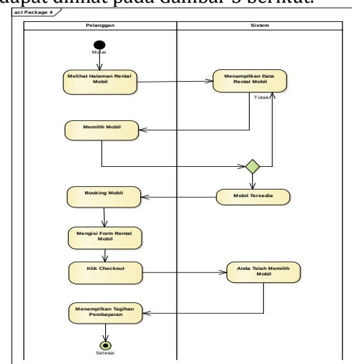
Gambar 5 Activity Diagram Rental Mobil
