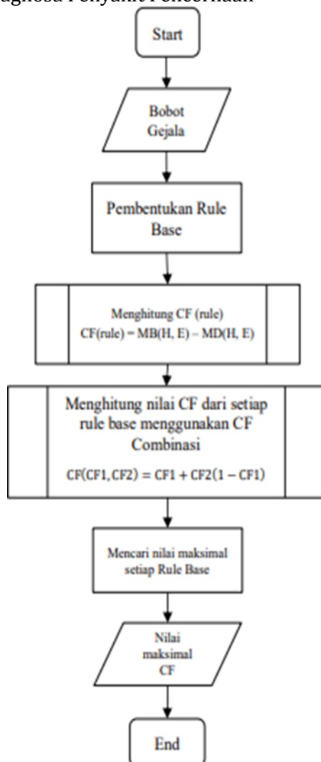
Gambar 4. Flowchart metode Certainty Factor
