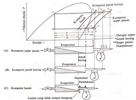
Gambar 5. Proses tertutupnya tube-shell Koil
