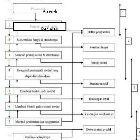
Gambar 1. Diagram Alir
