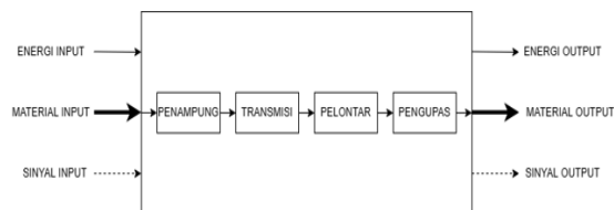
Gambar 9. Diagram Blok
