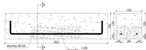
Fig. 7b BarChip in tension area of SRB
