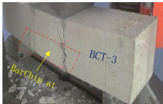
Fig. 10 Crack pattern of BCT-3
