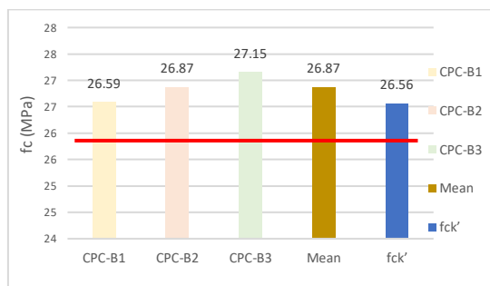
Fig. 6 Cylinder f_c' BarChip48
