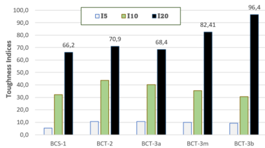
Fig. 13 Toughness Indices according to ASTM C108
