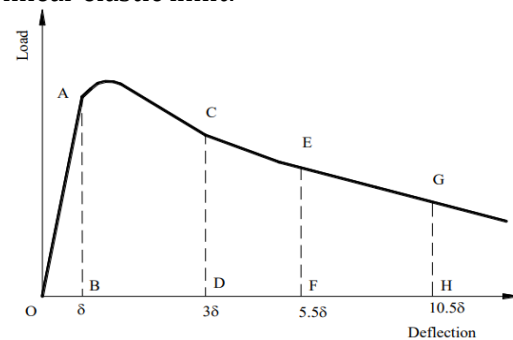
Fig. 8 Fracture toughness and Indices according to ASTM C1018
