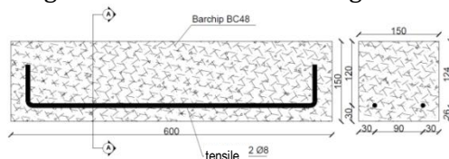
Fig. 7a BarChip in randomly oriented
