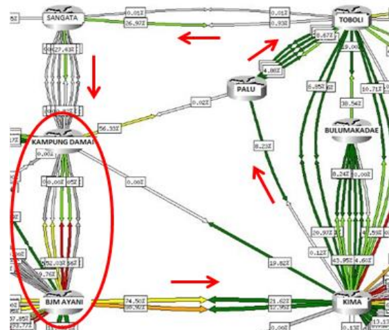
Gambar 14. Re-route LSP melalui jalur Toboli <> Sangata via Kimba
