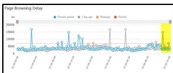
Gambar 18. KQI Delay Back to Normal After Balancing
