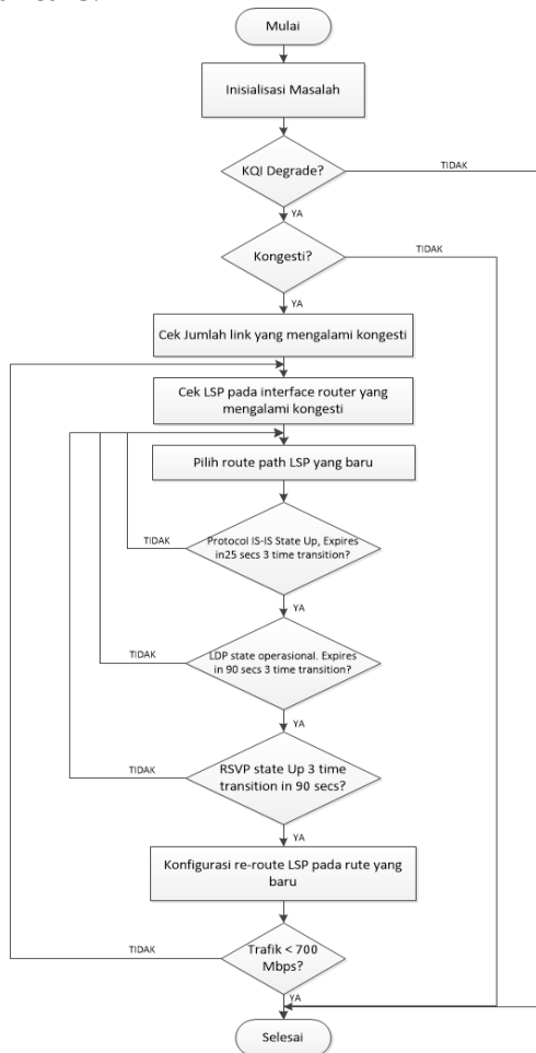
Gambar 8. Flowchart Re-Route LSP
