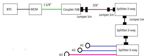
Gambar 3. Schematic Diagram Link Budget
