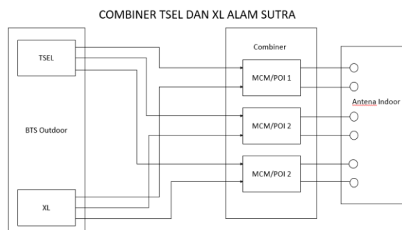
Gambar 2. Sistem Combiner Mall Alam Sutera
