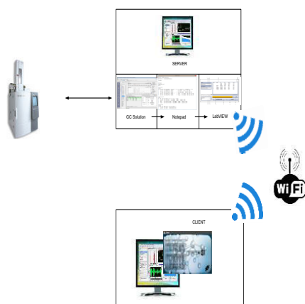
Gambar 3.1: Diagram Perancangan Program
