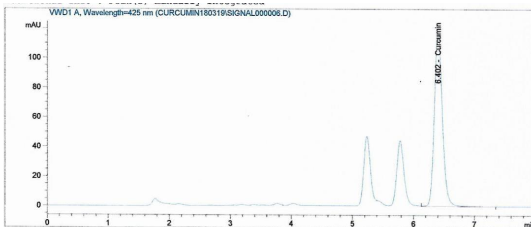
Gambar 5. Hasil kromatogram larutan sampel
