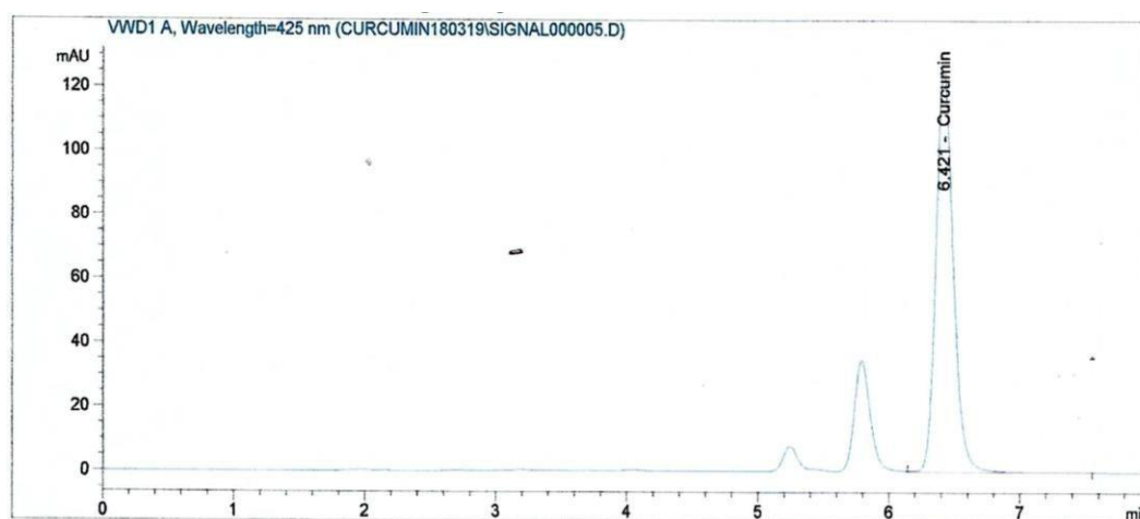
Gambar 6. Hasil kromatogram larutan baku 10 µg/mL
