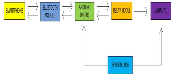
Gambar 3.1 Diagram blok system penelitian
