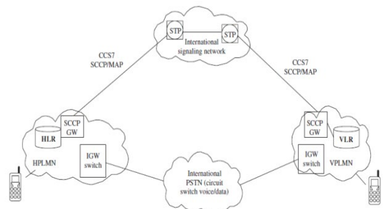
Gambar 4. Jaringan Global Roaming
